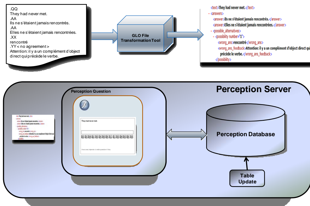
Figure 1 – Overview of the GLO process within QuestionMark™ Perception™
